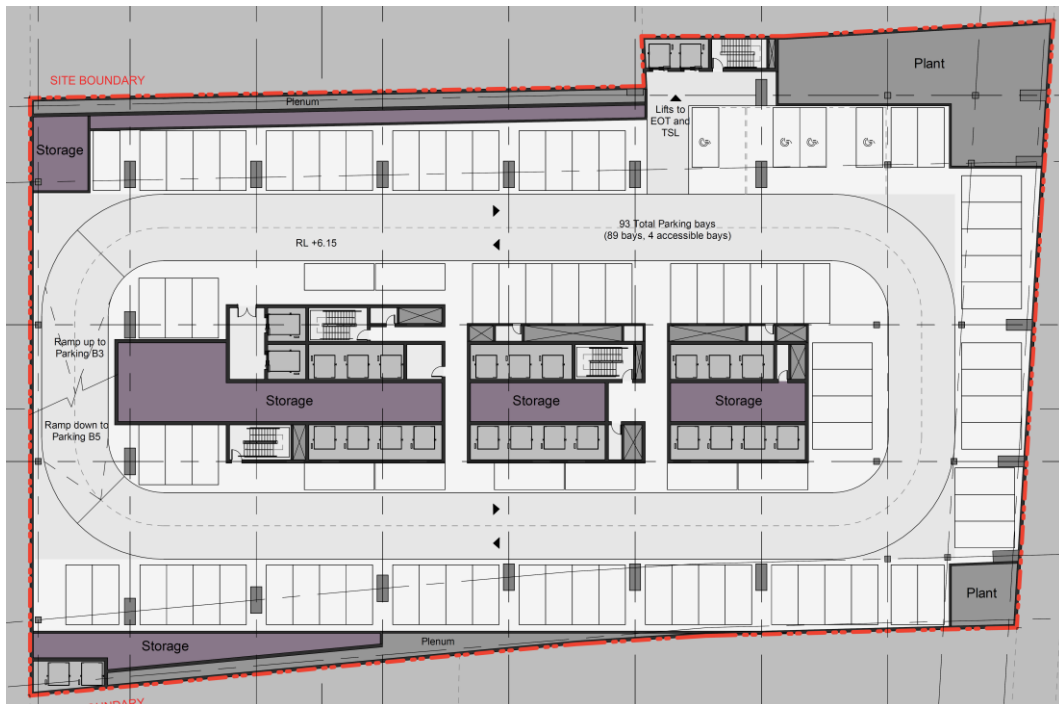
Figure 15: Parking layout – Basement 4 and 5
